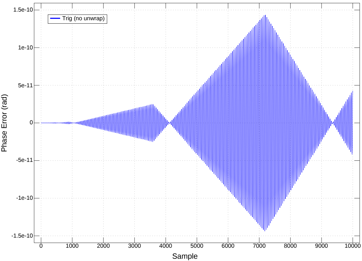
Trig Oscillator Phase Error vs Sample
