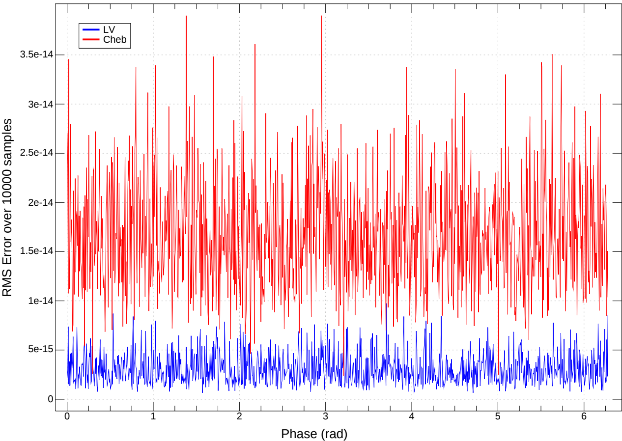
Magnitude RMS Error vs Initial Phase at 1000 Hz
