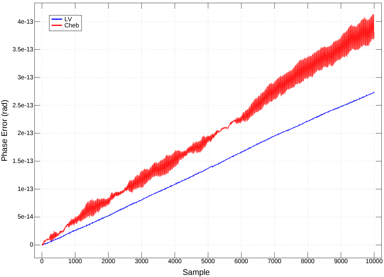
Oscillator Phase Error vs Sample
