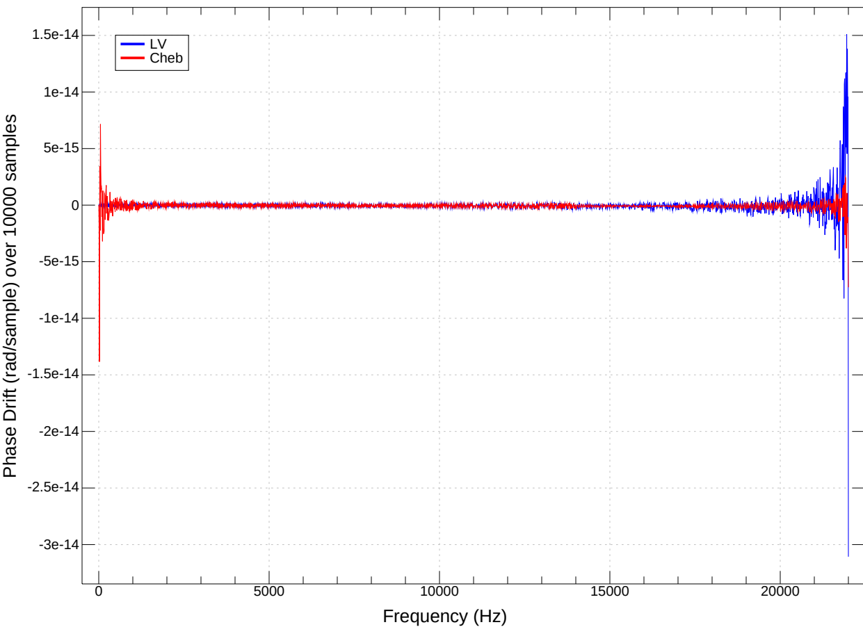
Oscillator Phase Drift vs Frequency
